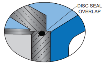
Figure 4 - Resilient Seating Detail at High Pressure
