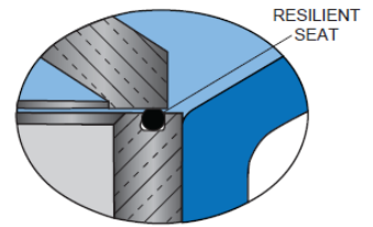
Figure 3 - Resilient Seating Detail at Low Pressure
