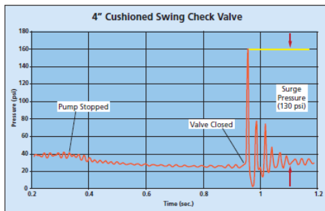
Figure 1 - Cushioned Swing Check Valve Dynamic Test Results
