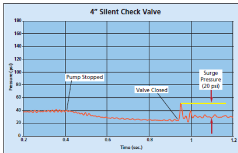
Figure 2 - Silent Check Valve Dynamic Test Results
