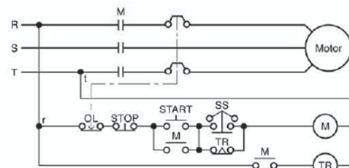
Figure 2 Example of circuit for slip detection and overload detection
